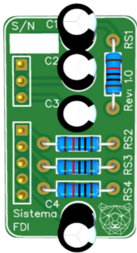
TOP PCB VIEW
